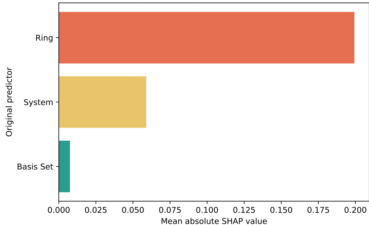
Grouped SHAP importance: norm, Q2(1)zz
